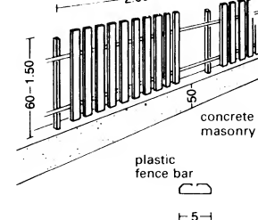
㉓ Steel profile fence (galvanised) with plastic fencing bars
